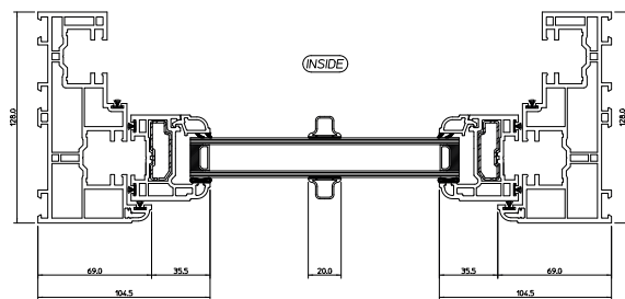
Downwards View - Top Sash
