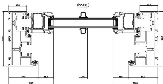
Downwards View - Bottom Sash
