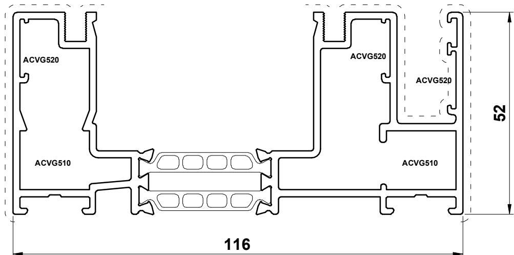
VG511 Two Track Outer Frame with Upstand
