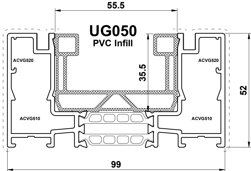
VG510 Two Track Outer Frame
