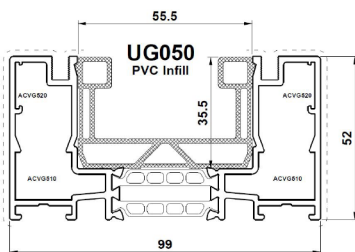
Two Track Outer Frame
